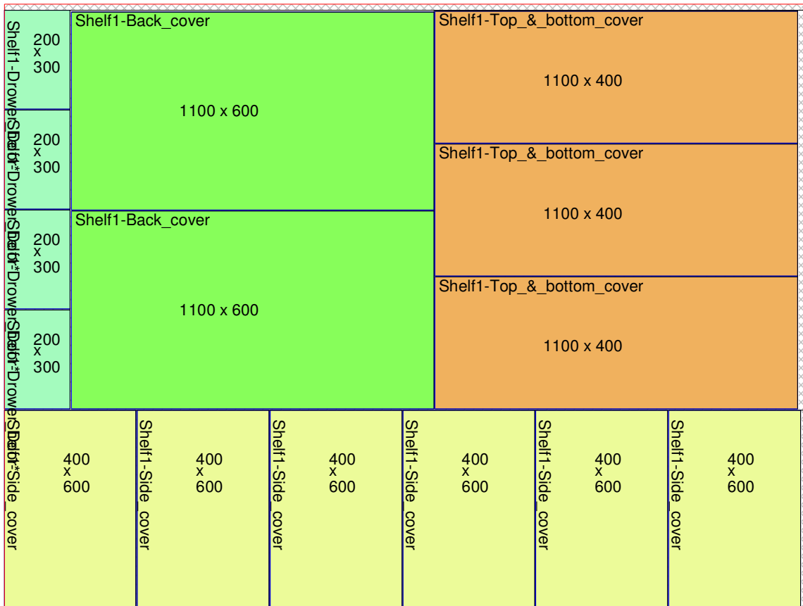
Layout 4 of 4(Stock:Stk2 Dim:2440 x 1830 Qty:5 Material:mdf Thk:12)
