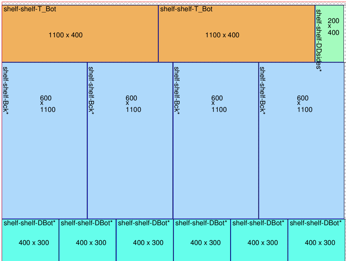
Layout 7 of 9(Stock:stk2 Dim:2440 x 1830 Qty:65 Material:mdf Thk:10)
